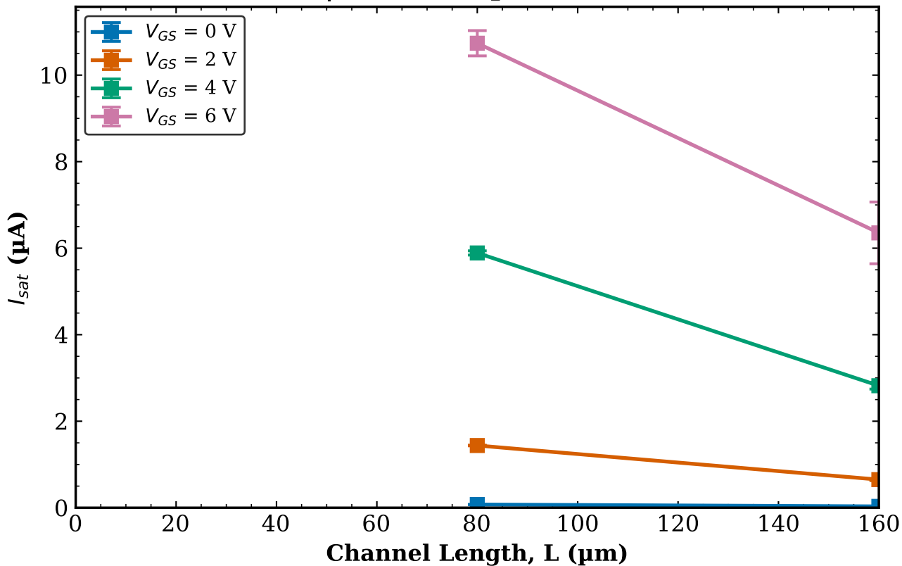
TFT2 Combined (Tr. 1 & 2) I_{sat} vs L | W = 100 \mu\text{m} (mean \pm std)
